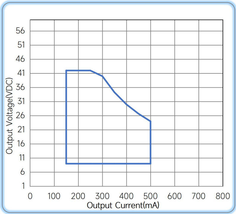
Operating window 100%
